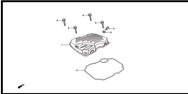
E-2-2 CULATA 150EVO
