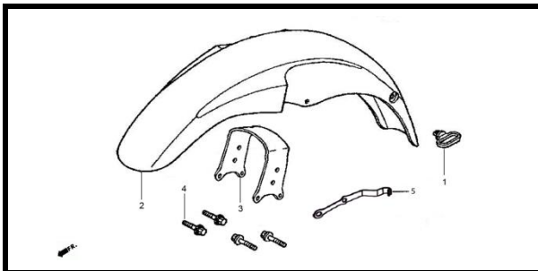
F-7 GUARDABARRO DELANTERO
