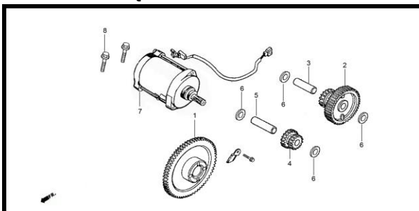
E-15 ARRANQUE
